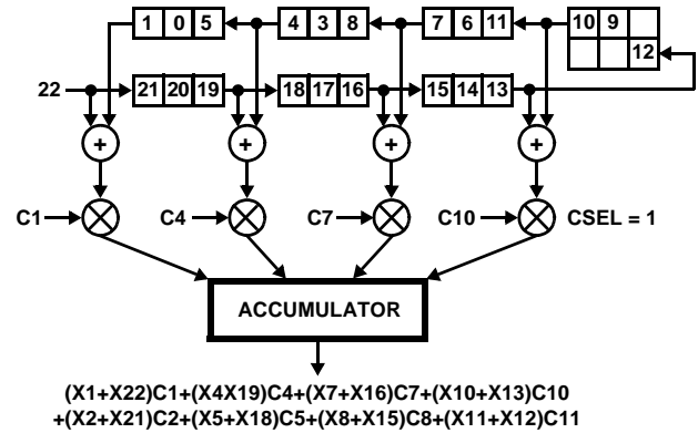
FIGURE 17B. COMPUTATIONAL FLOW AS DATA SAMPLE 22 IS CLOCKED INTO THE FEED FORWARD STAGE
